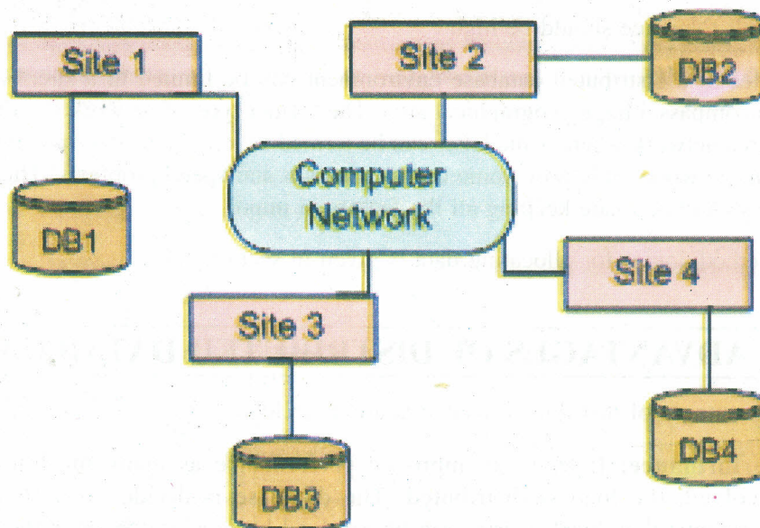
Fig. 1: Distributed Database
