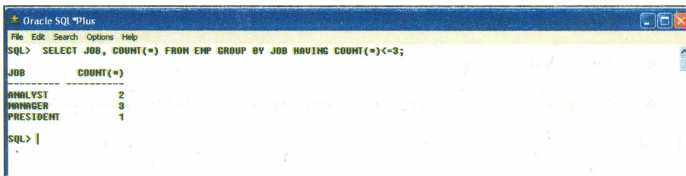
Fig. 33: Having Clause
