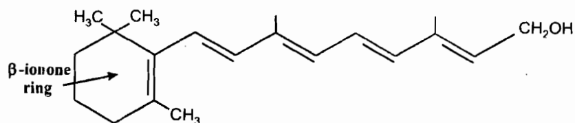
(a) Retinol
