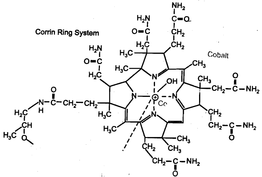
(a) Cyanocobalamin
