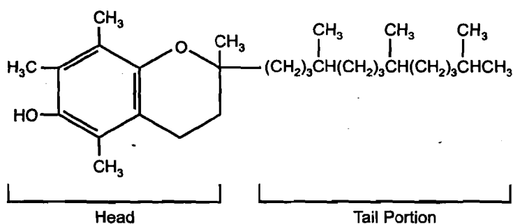
Figure 3.15: \alpha -tocopherol
